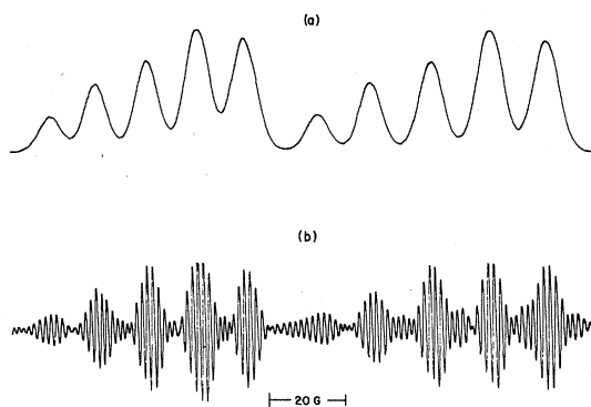
FIG. 2. (a) Boxcar tracing of a portion of the CdS : Mn spectrum with the boxcar gate set on the electron spin-echo signal. The angle between the CdS c axis and the Zeeman field is 28^\circ . The microwave field intensity H_1 was 0.5 G. (b) Boxcar tracing of the same portion of the CdS : Mn spectrum with the boxcar gate set on the satellite S following a single microwave pulse. The period of the oscillation is \sim 1.4 G. The microwave field intensity H_1 was 1.5 G. Values of H_1 \sim 6 G (as used in other experiments) yield a similar trace, but the resemblance to the normal EPR spectrum (a) is partially obscured on account of the excitation of more than one EPR line at a time.
